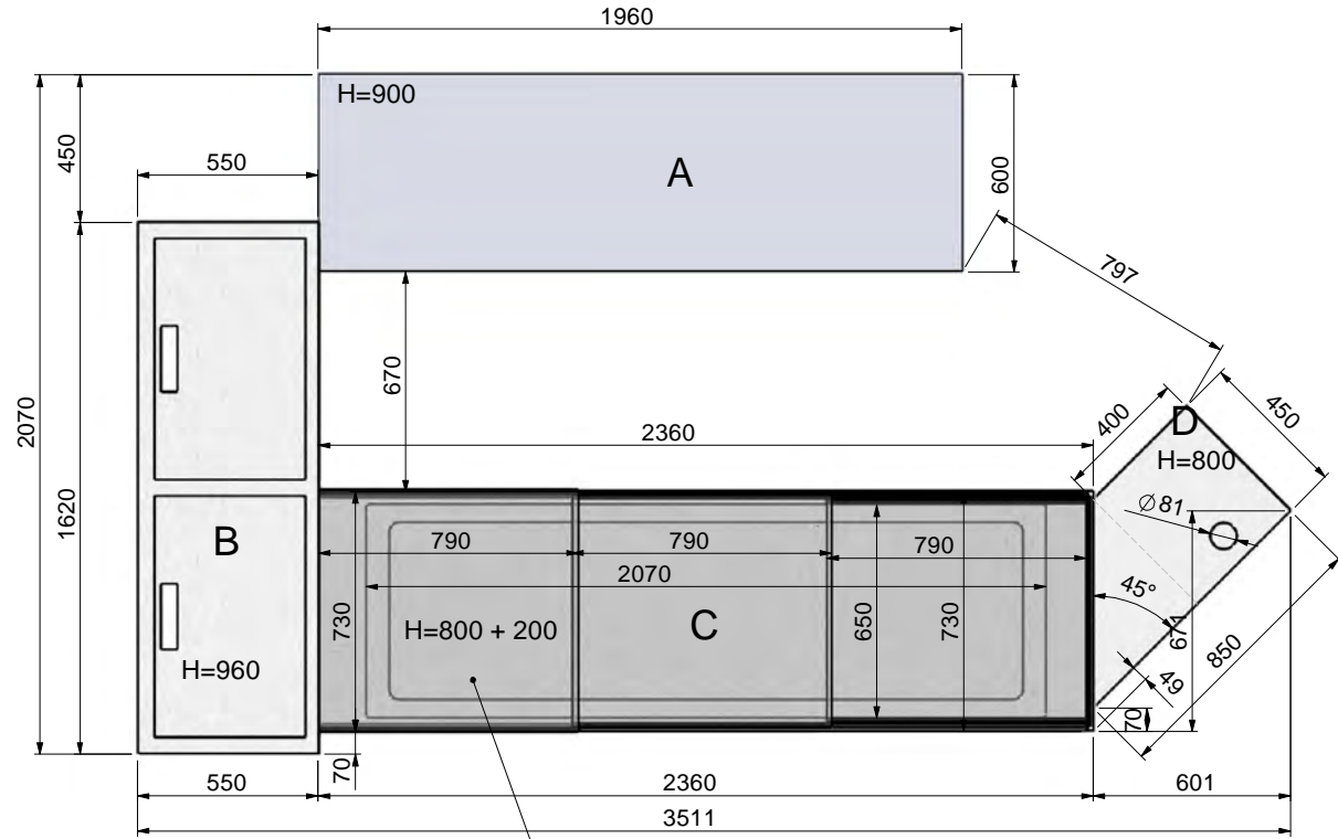
PLAN REFRIGEREE DEINOX AR6GPR1L
